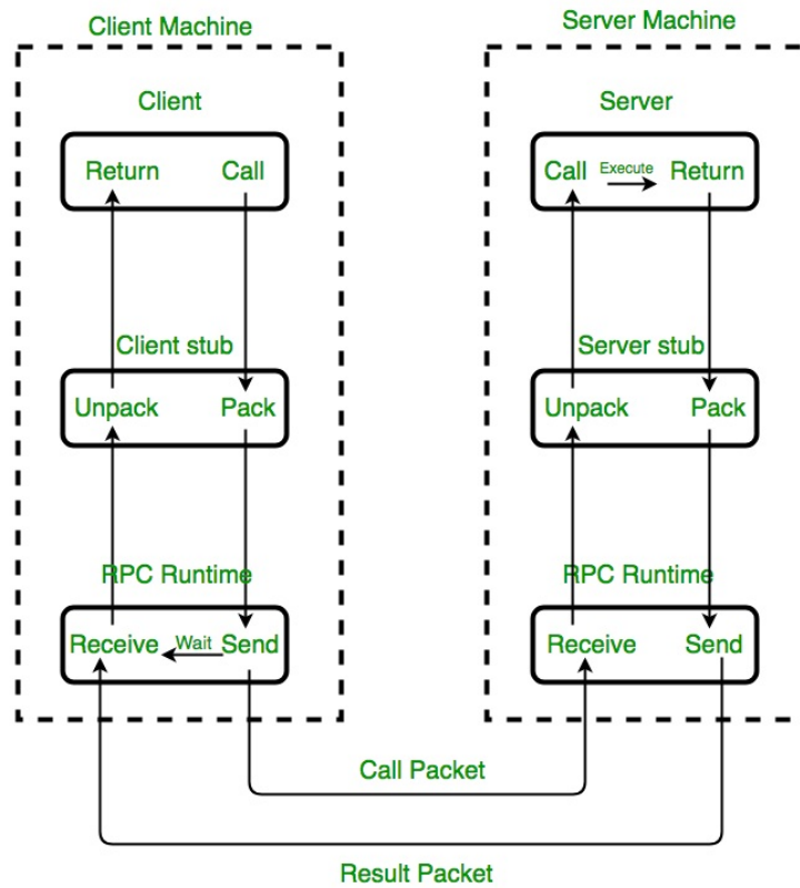
Implementation of RPC mechanism
