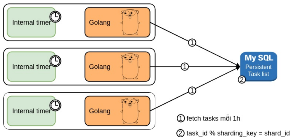
Distributed Task Distribution
