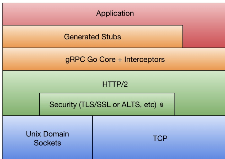
gRPC technology stack
