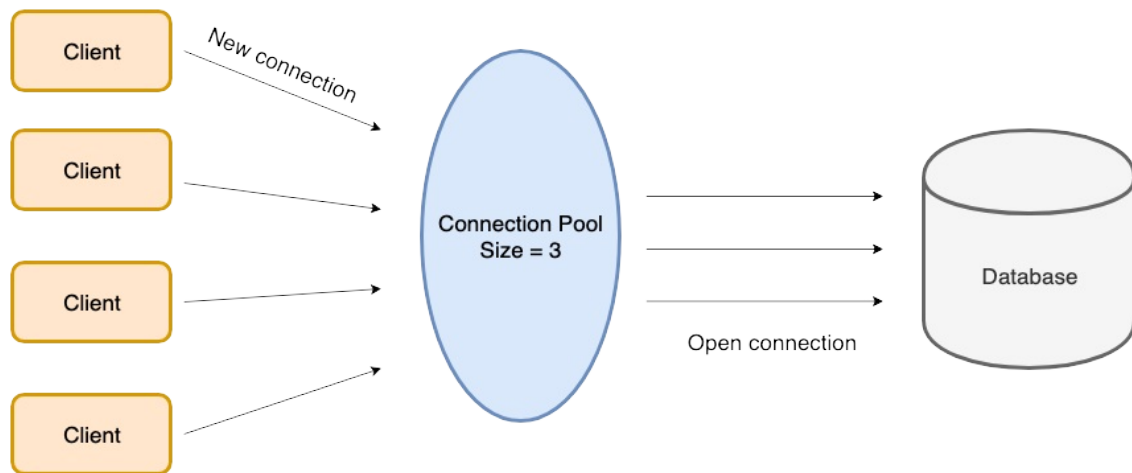
Minh hoạ Connection Pool
