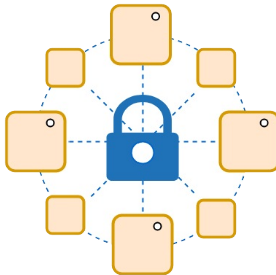
Distributed lock
