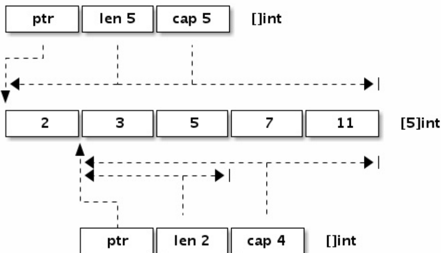
Slice layout
