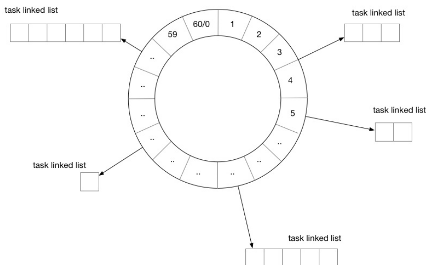
Time Wheel
